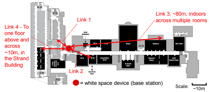
Fig. 3. Indoor room plans of the Strand and King's buildings (combined) of the King's College London Strand Campus. The Strand Building is to the left of the WSD, and the King's Building is to the right. Both the 1 st and 2 nd floors of the Strand Building are depicted, whereas only the 2 nd floor of the King's Building is depicted.
